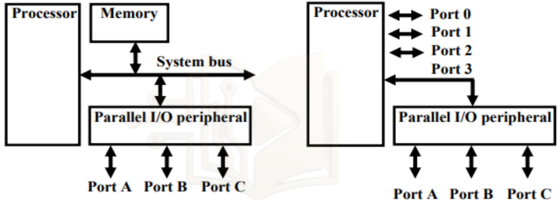
Adding parallel I/O to a bus-based I/O processor
