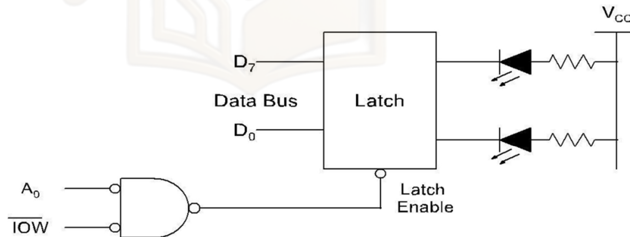
Fig: Non unique Address Decoding
